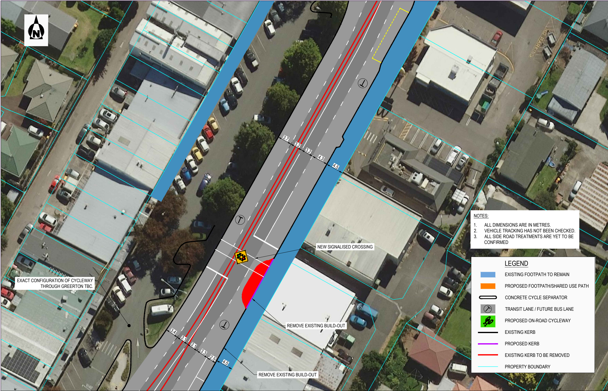
CAMERON ROAD STAGE 2 OPTION 3 - TRANSIT AND CYCLE SHEET 22: GREERTON CROSSING
