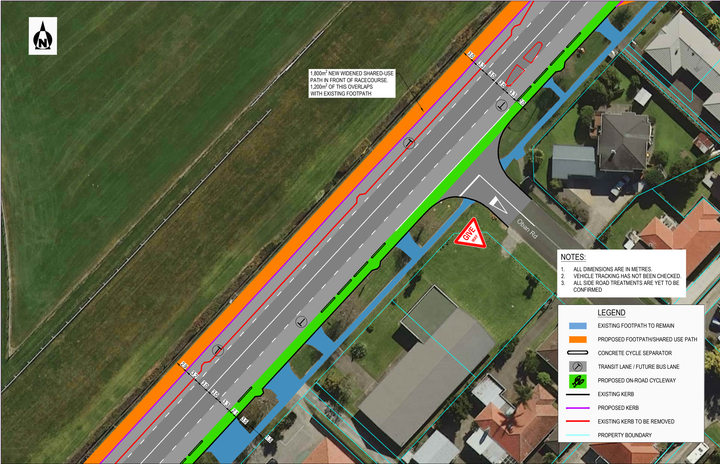
CAMERON ROAD STAGE 2 OPTION 3 - TRANSIT AND CYCLE SHEET 26: OBAN ROAD
